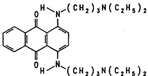
Compound 1b
